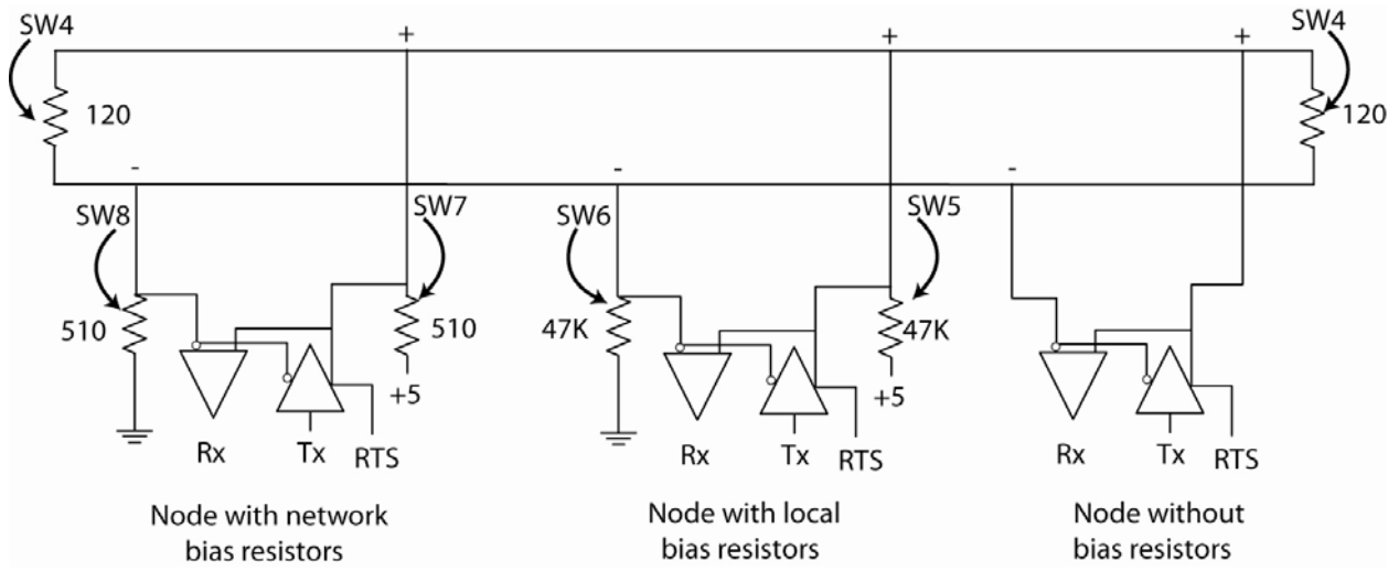
Figure 5. Bias Resistors
