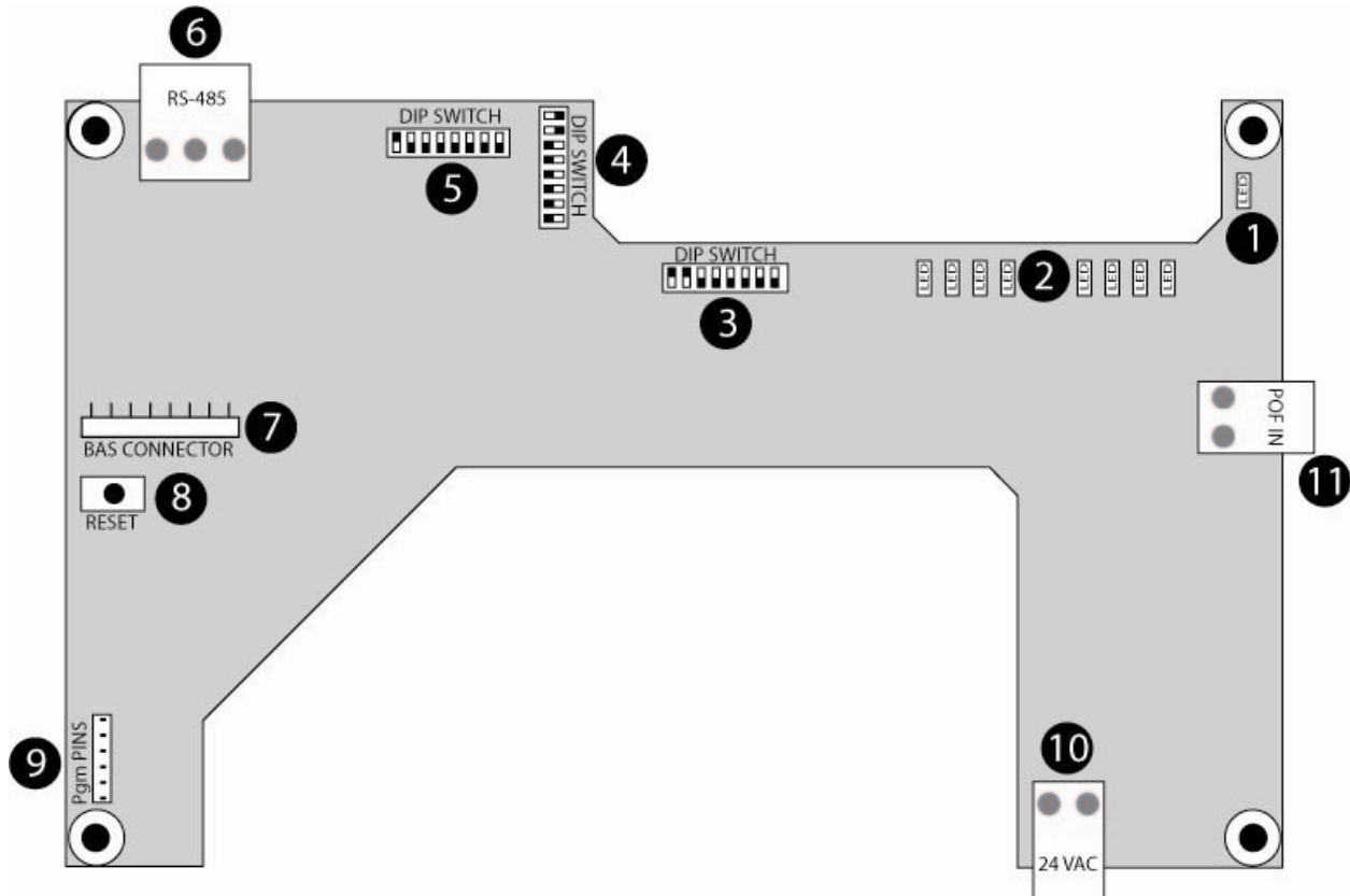
Figure 1. Board Layout
